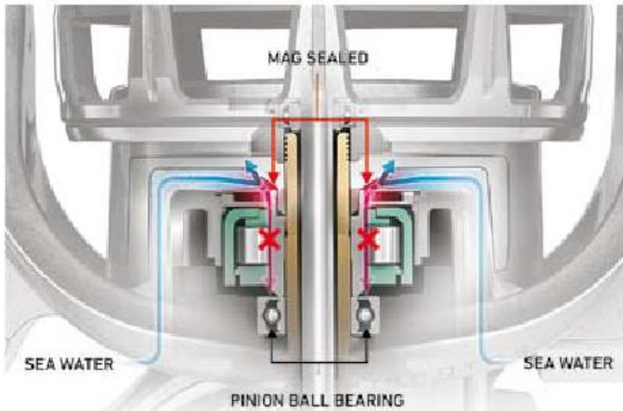
Comparison of reels with/without MAG SEALED. Source: DAIWA Intern. Service Dept.
