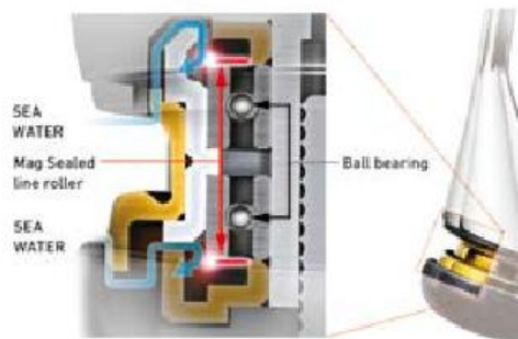
Reels with/without MAG SEALED line roller. Source: DAIWA Intern. Service Dept.
